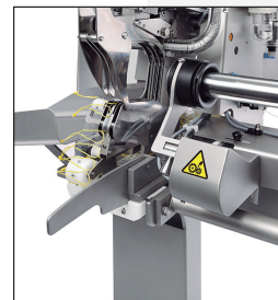
Filling tube's movement to ensure the clip is in the center of the sausage with a minimum effort.
