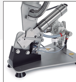
Accessories: automatic knife, pressure reducer with filter & lubricator, and tabletop feet.
