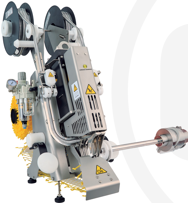
Clip on spool for a faster production.
